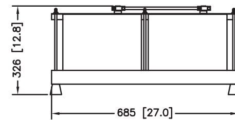
BATTERY & BATTERY RACK SCALE: 2X
