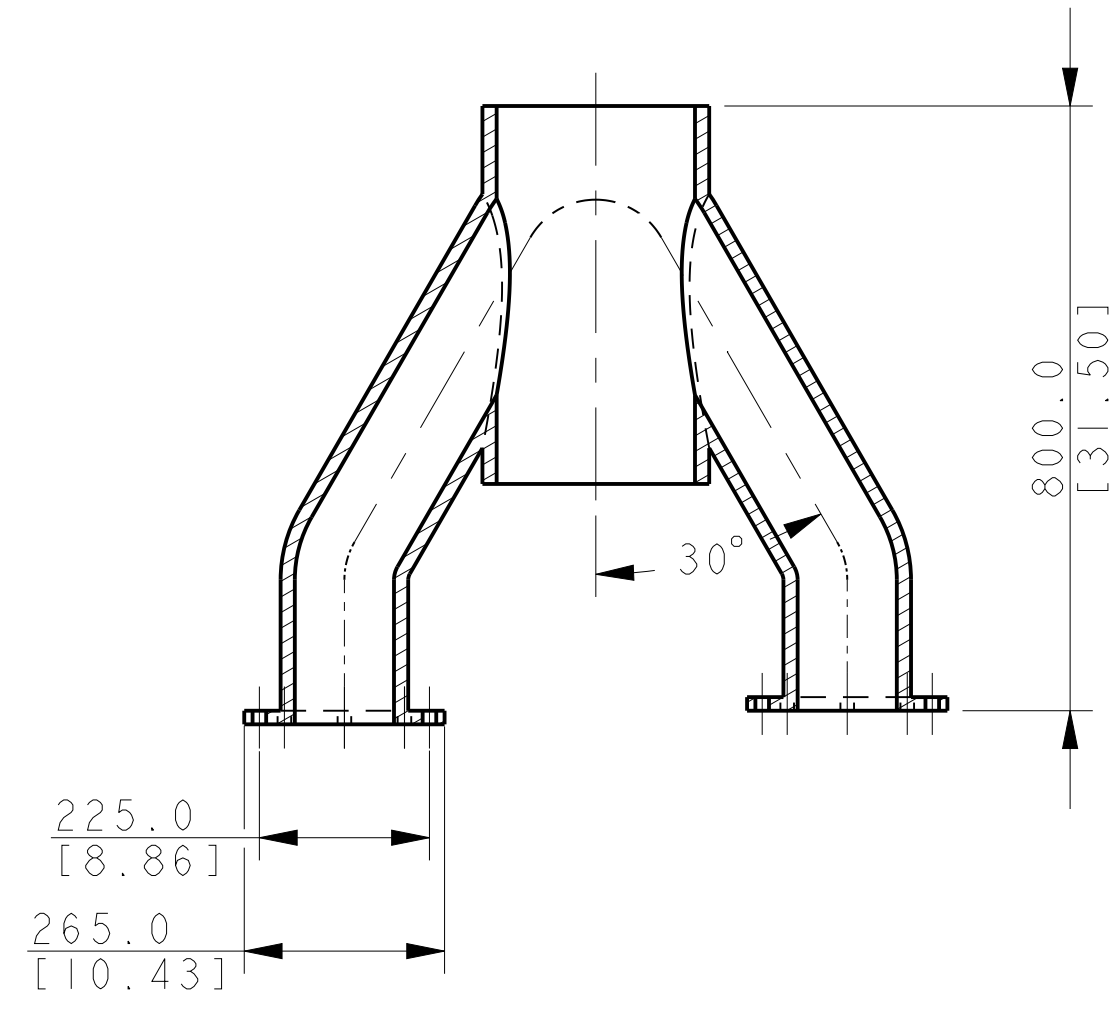
V-ENGINE EXHAUST Y-PIPE
