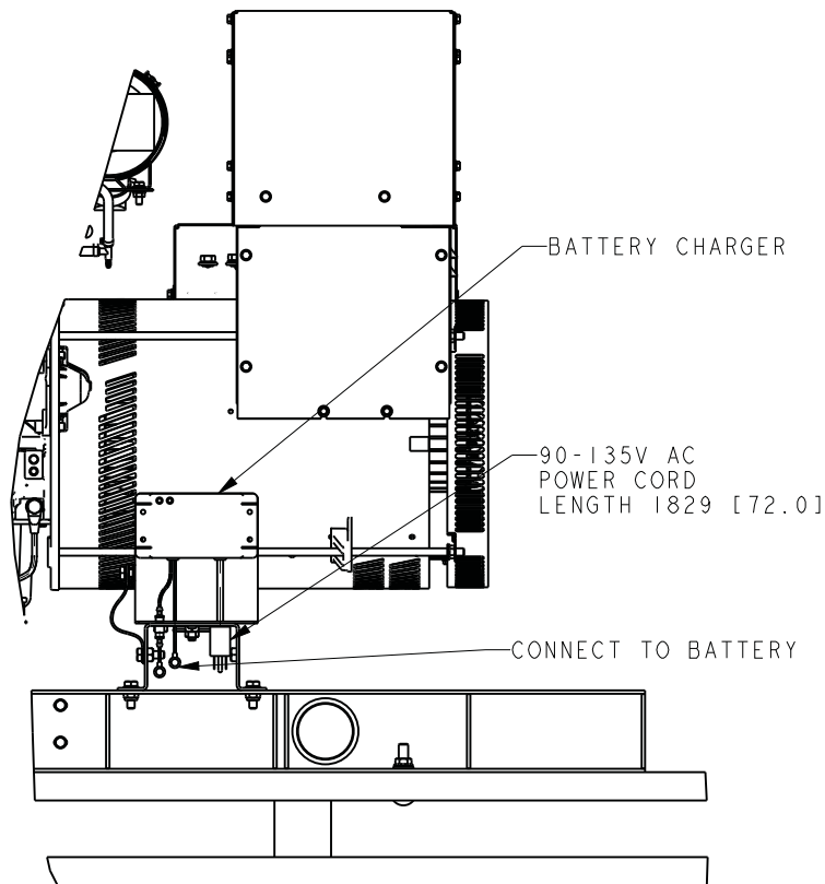
BATTERY CHARGER
