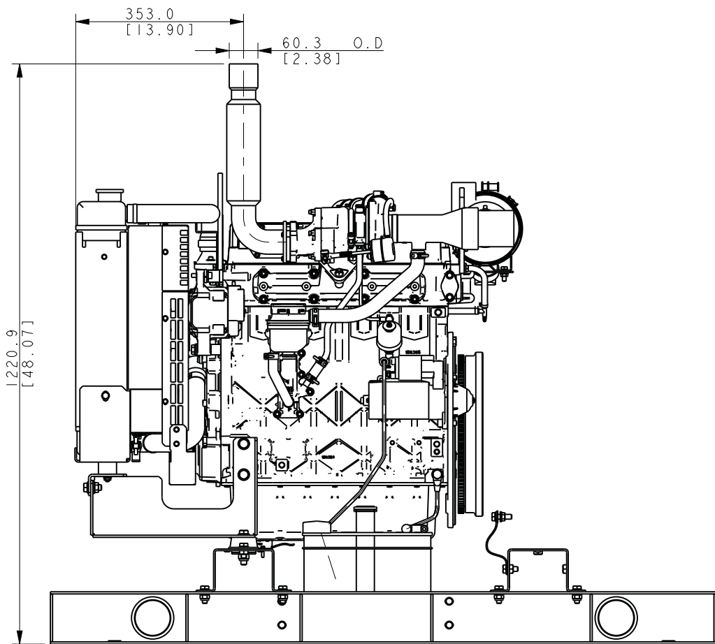
FLEXIBLE EXHAUST
