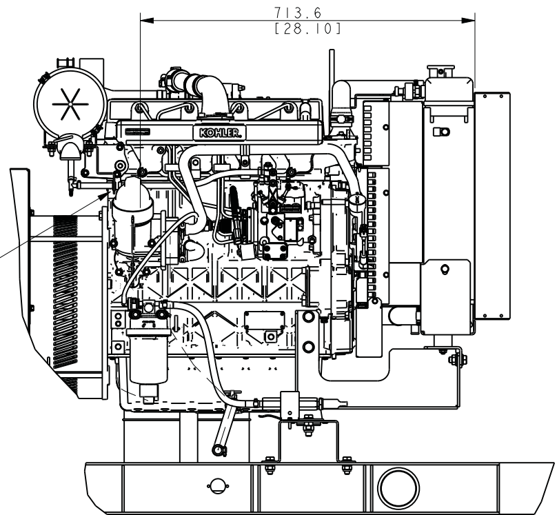
BLOCK HEATER
