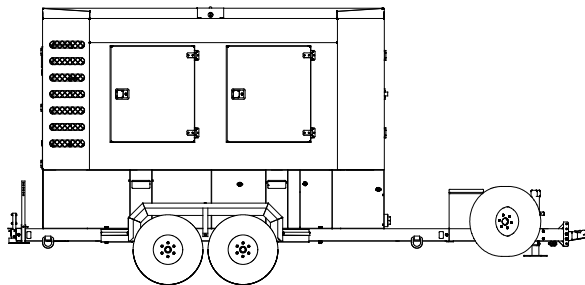
Standard Skid Model with Available Options
